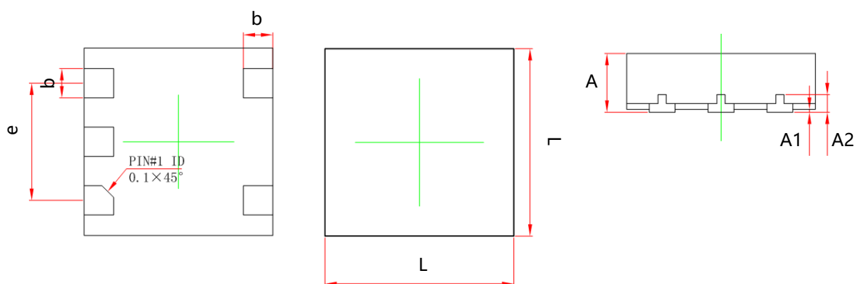
Figure.18 DFN1616 Package Drawing
